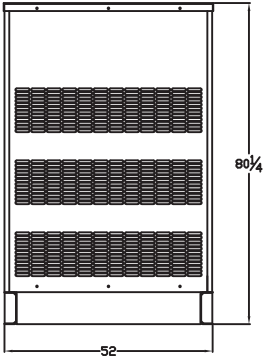
GENERATOR END VIEW
