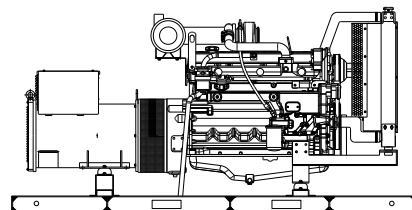
“OPEN” GEN-SET
