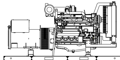
“OPEN” GEN-SET
