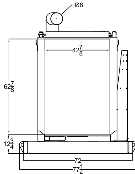
RADIATOR VIEW
