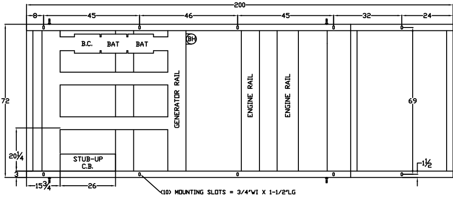
FRAME VIEW
