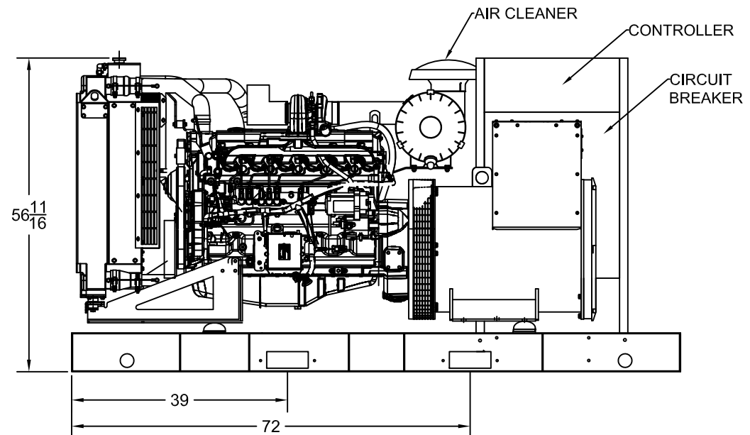
SIDE VIEW
