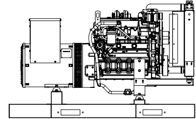
"OPEN" GEN-SET
