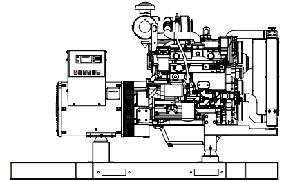
"OPEN" GEN-SET
