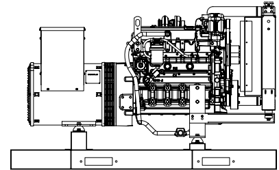
"OPEN" GEN-SET
