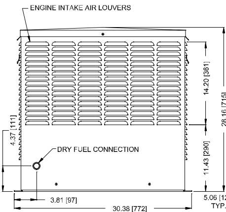
ENGINE END VIEW
