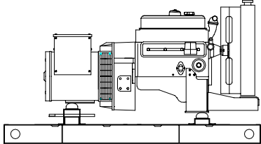
"OPEN" GEN-SET
