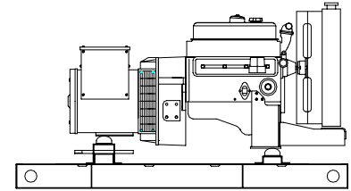
"OPEN" GEN-SET
