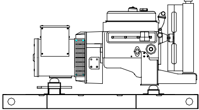
"OPEN" GEN-SET
